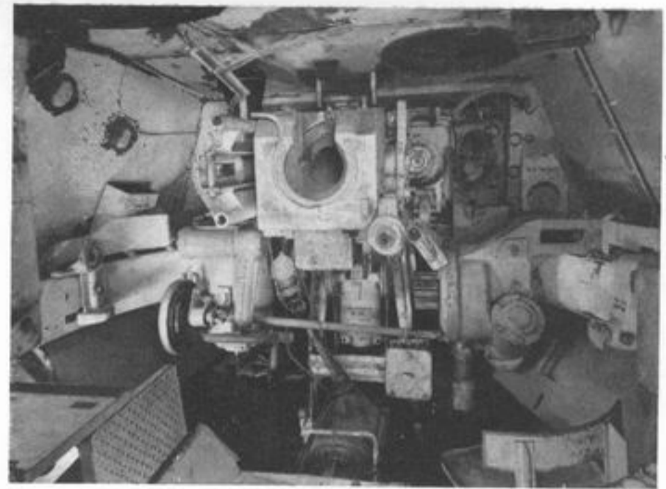
Inside the Panther turret, showing loader's seat (right) and the elevating and traversing handwheels (left, centre). (IWM)
