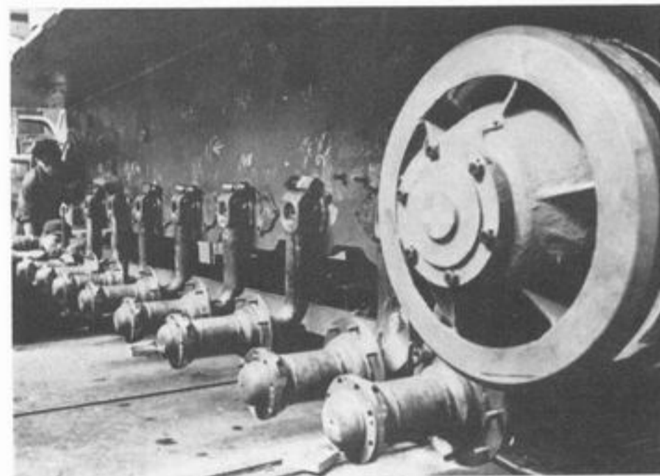
The radius arms from the axles were attached to the torsion bars running across the hull floor. In this view can also be seen the anchorage points for the alternate torsion bars from the opposite axles. (IWM)
