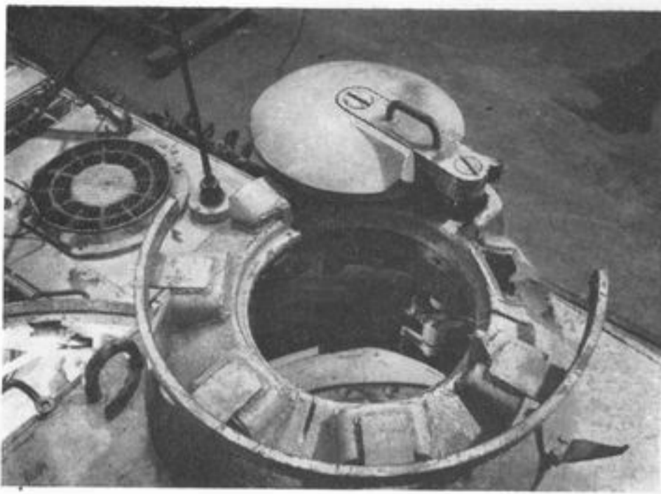
A close view of the cupola in the Panther Ausf A, showing the armoured periscopes (one has been shot away), the gun ring, and the horizontally opening hatch. (IWM)
