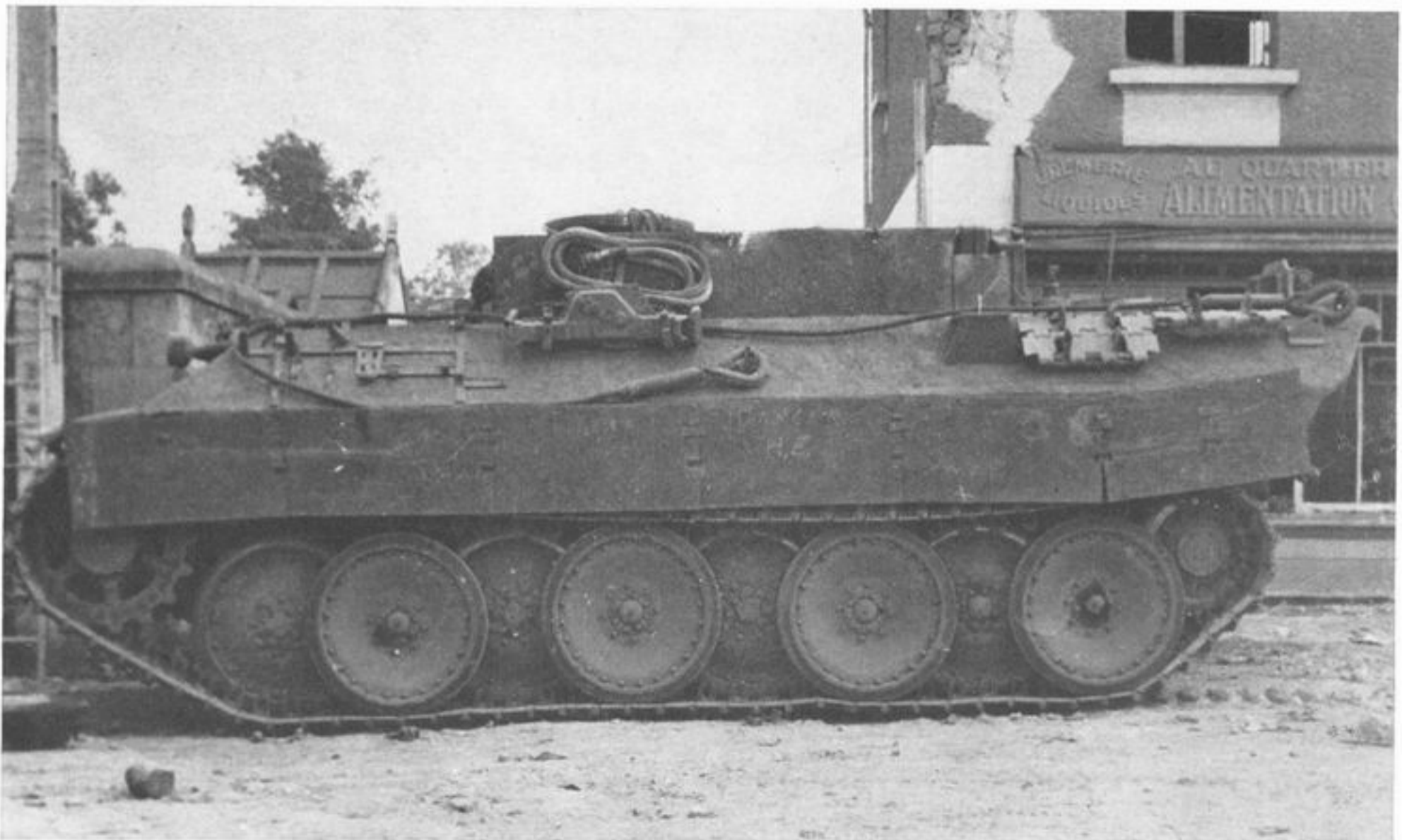
Not all Bergepanthers were fitted with earth spades. They were used as towing vehicles only. Others had the winch removed and were used as munitions carriers. (IWM)
