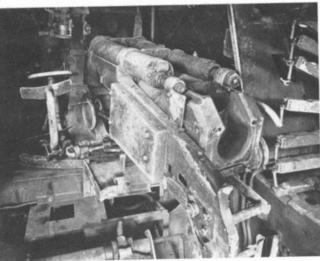
8.8 cm. gun breech, driver's seat (left), and telescope sight (top left) inside a Jagdpanther. (IWM)
