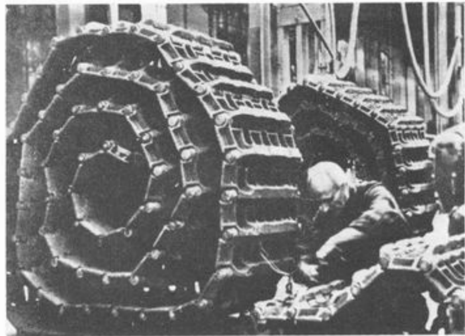
The Panther's tracks, heavily ribbed specially for running on ice, had 86 shoes on each side.
