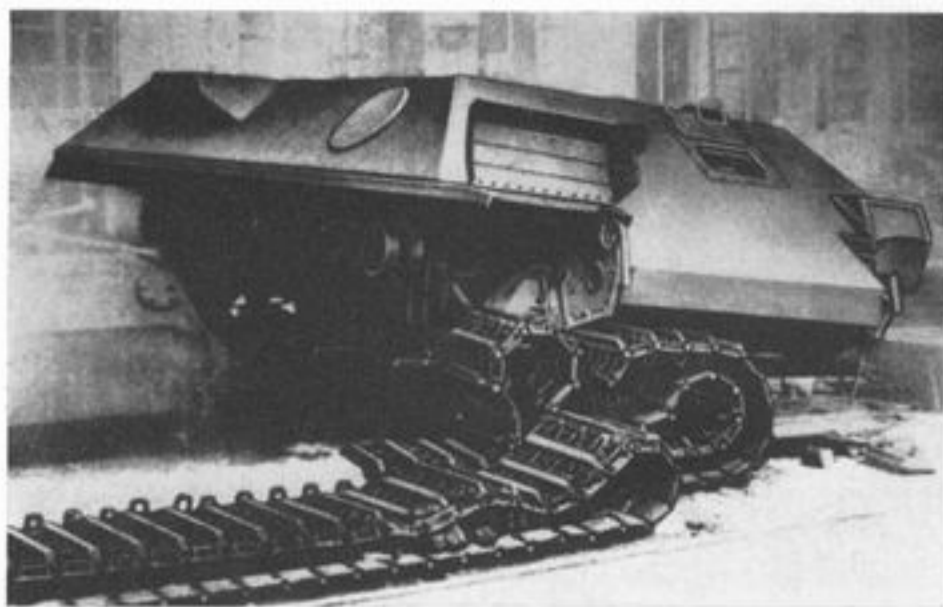
One of the uncompleted VK.3002(DB) prototypes. Unlike the T-34, this vehicle had return rollers. Resemblance to the T-34 is particularly striking in this front view.
