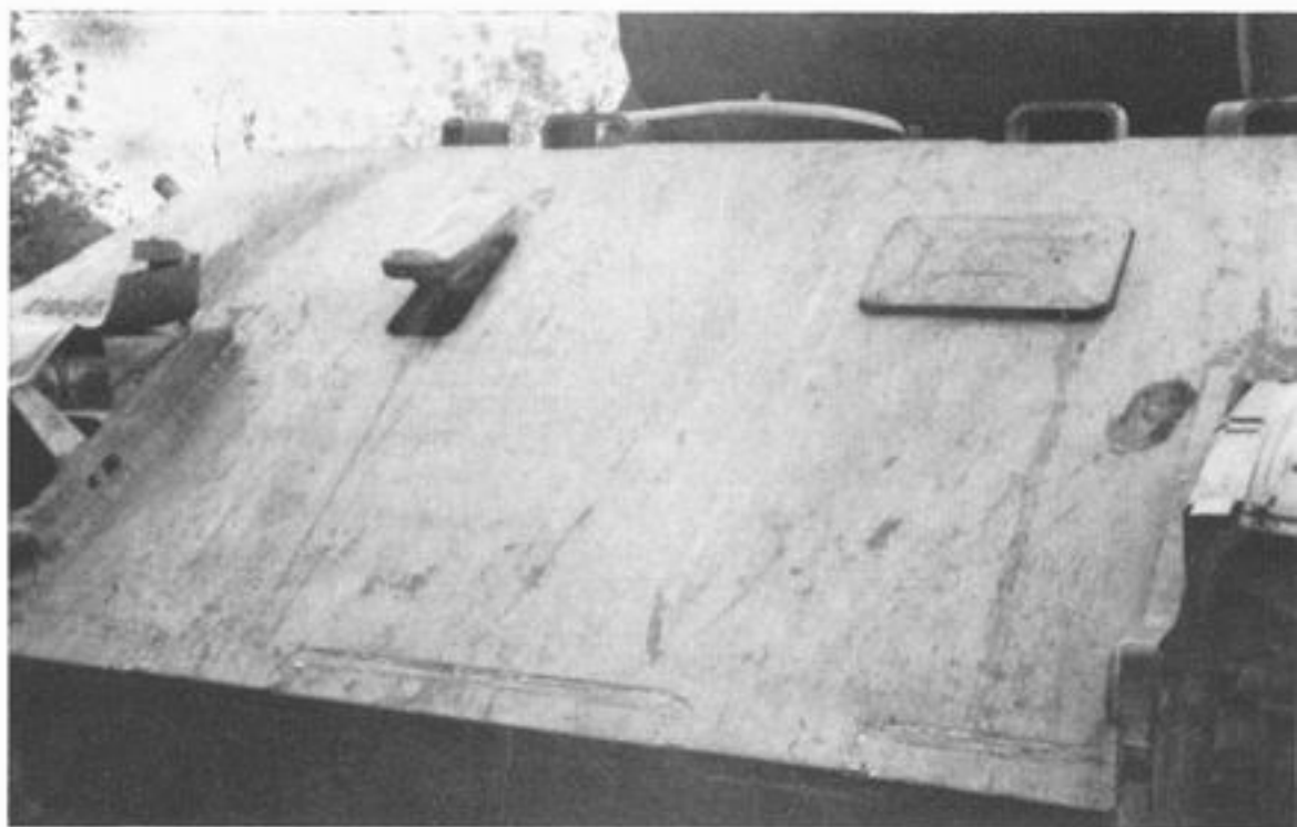
Close up of a Panther Ausf D glacis plate shows the driver's vision port (closed), the machine-gun flap, the episcopes on the front decking, the mortised welded joints and the chassis number painted above the right dustguard. (IWM)
