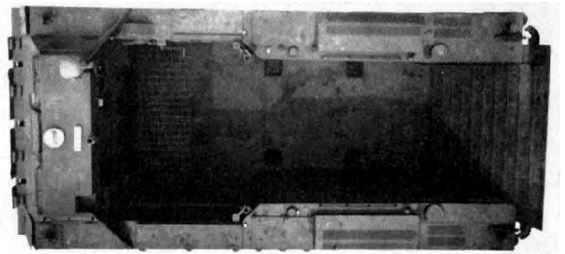
Top view of LVT 3 showing increase in cargo space achieved by placing engines in side pontoons.
