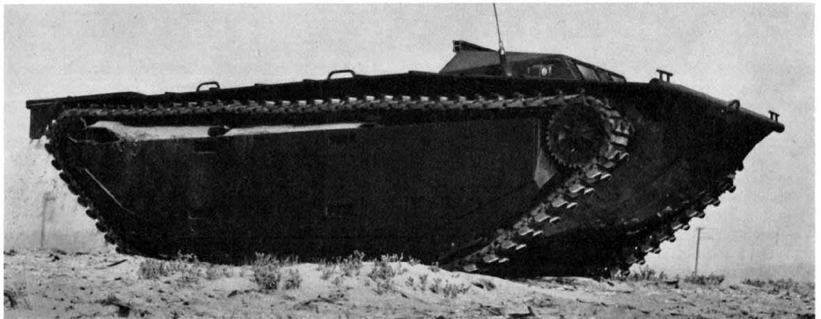
LVT 2 equipped with radio and showing bumper welded to bow.
