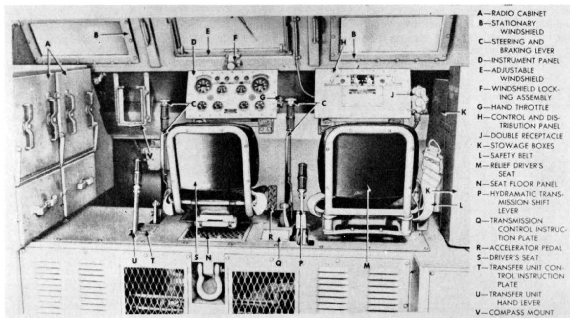
Driver's position in LVT 3 showing location of steering levers and other controls (Protective shield has been removed).
