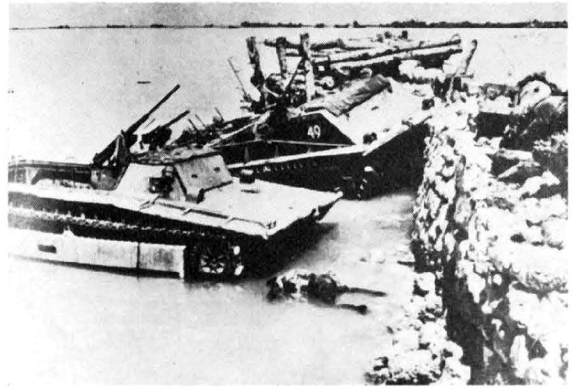
Knocked-out LVT 1 and LVT 2 on the beach at Tarawa following the initial assault. (Photo: U.S. Marine Corps)
