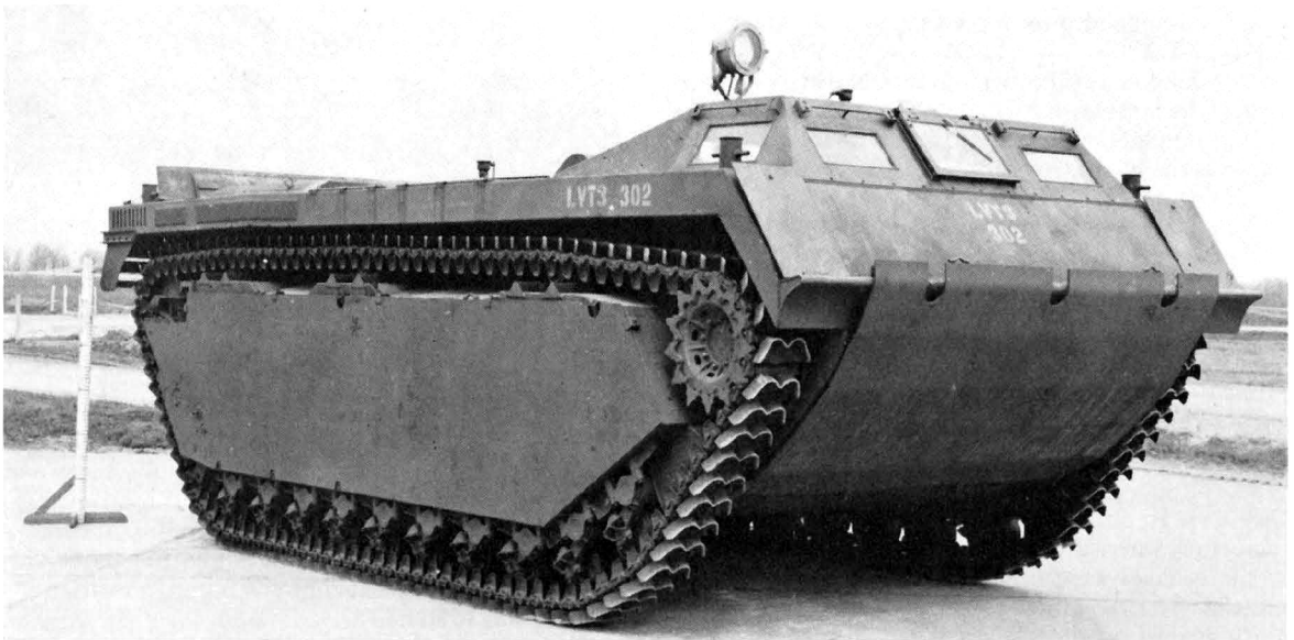
LVT 3 with supplementary or bolt-on armor installed over the bow and the side pontoons.
