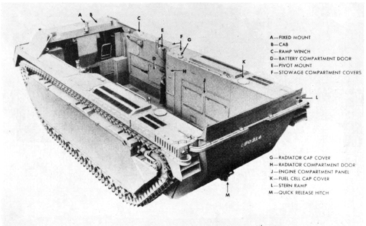
Three-quarter left top view of LVT 3 showing protective plate for driver and with bolt-on armor installed.
