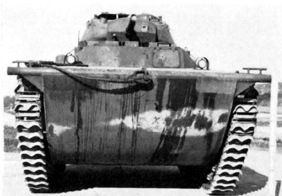
Front view of LVT (A) 1 mounting an M24 Light Tank turret in place of M3 Light Tank turret. (Photo: U.S. Ordnance Dept.)
