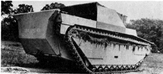
LVT 4 experimentally fitted with a 20 tube 7.2-in. T54 Rocket Launcher.
