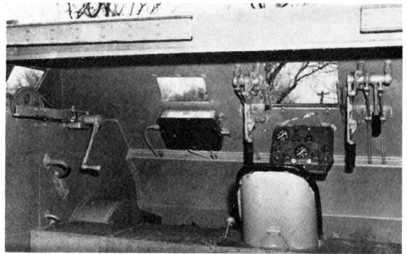
Driver's seat in LVT 4 showing difference in location of steering levers as compared with the LVT 3. (Photo: Food Machinery Corporation)
