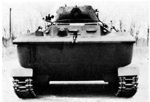
Bow of LVT (A) 5 in post-World War II modification by Continental Aviation & Engineering Corporation also showing new type of track.
