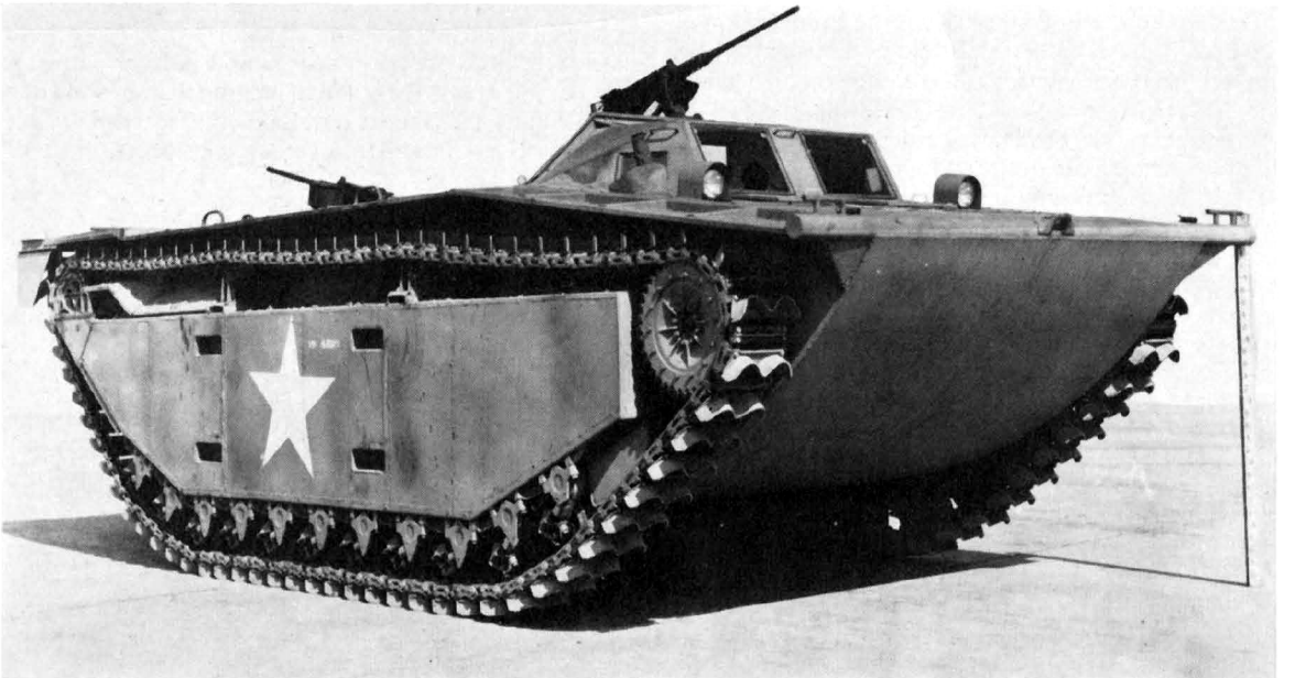
LVT 2 showing new W-shaped grousers and Torsilastic suspension system.
