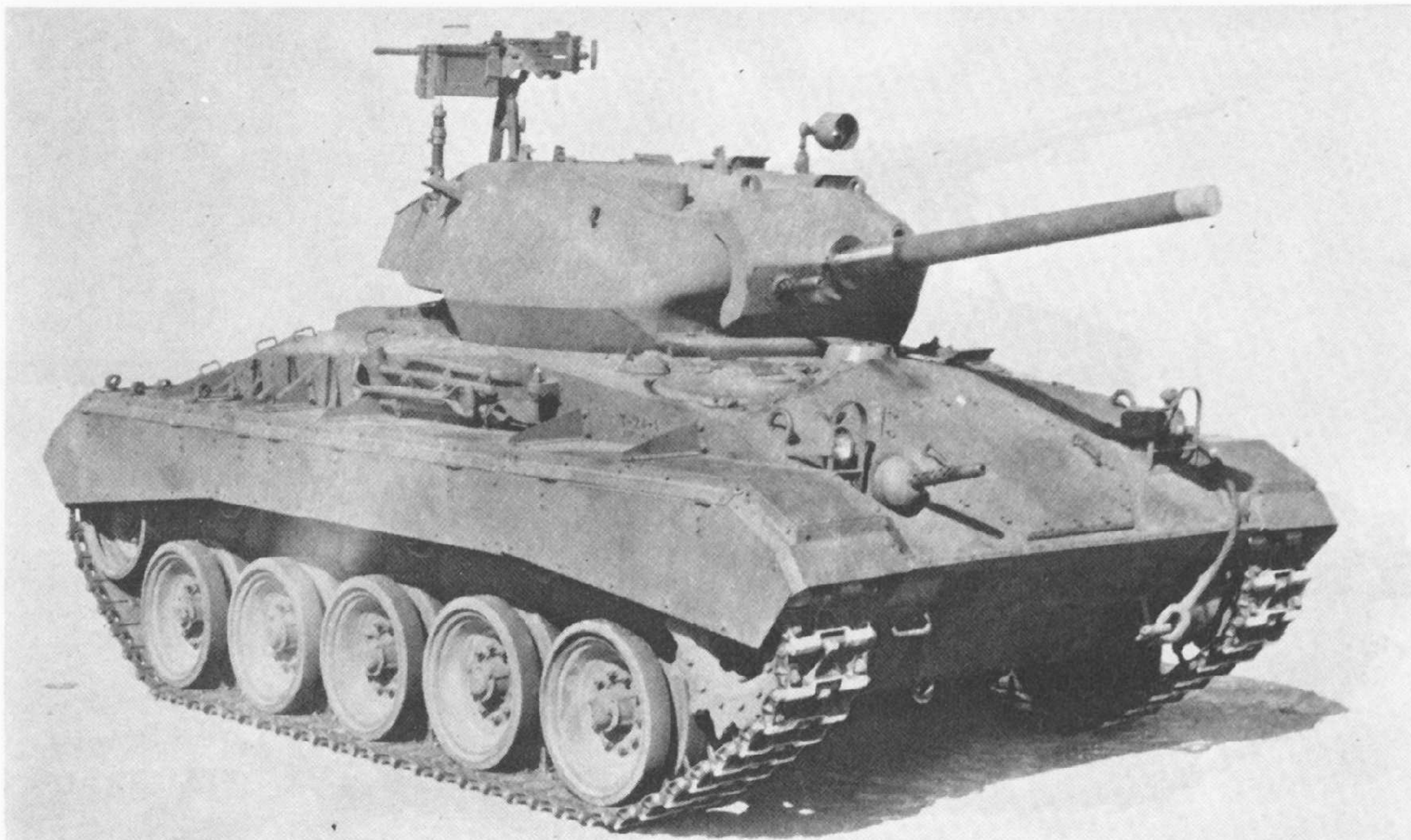
Pilot model of T.24 light tank, 1943.
