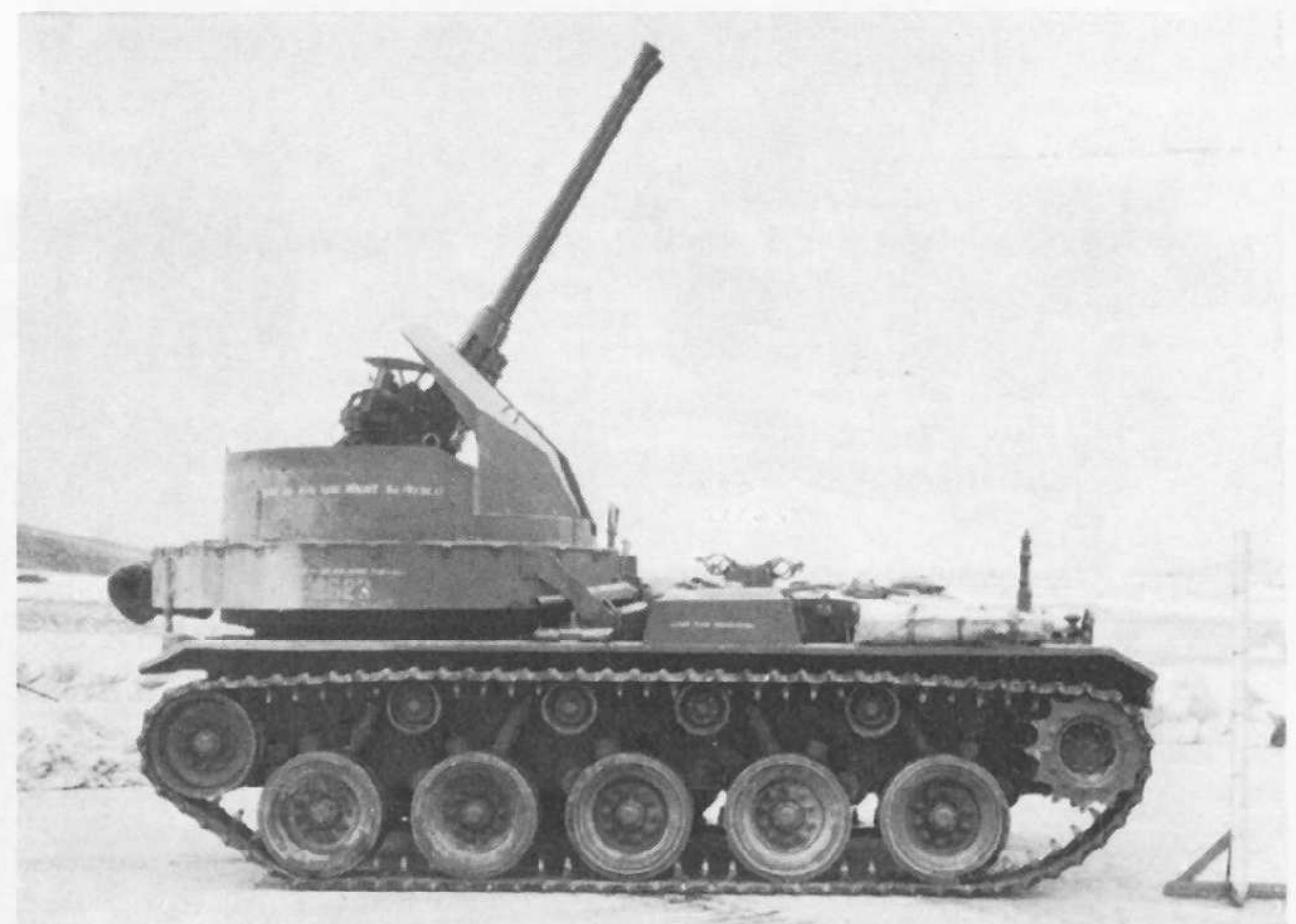
M.19 (T.65 E1) twin 40 mm. Gun motor carriage. (Photo: Icks collection)
