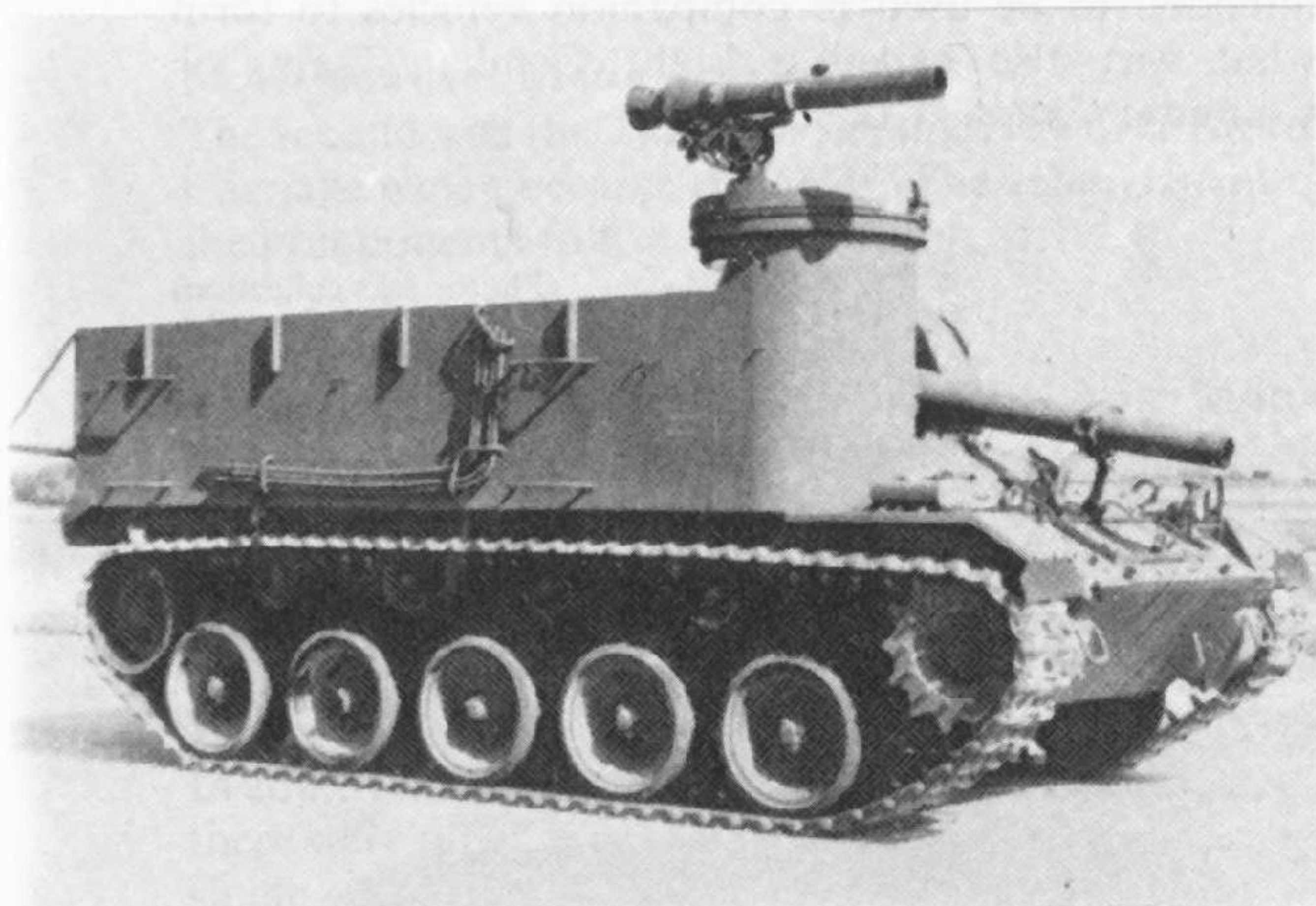
M.37 (T.76) 105 mm. Howitzer motor carriage with 4.2 in. recoilless mortar substituted for .50 cal. pupil machine-gun.
