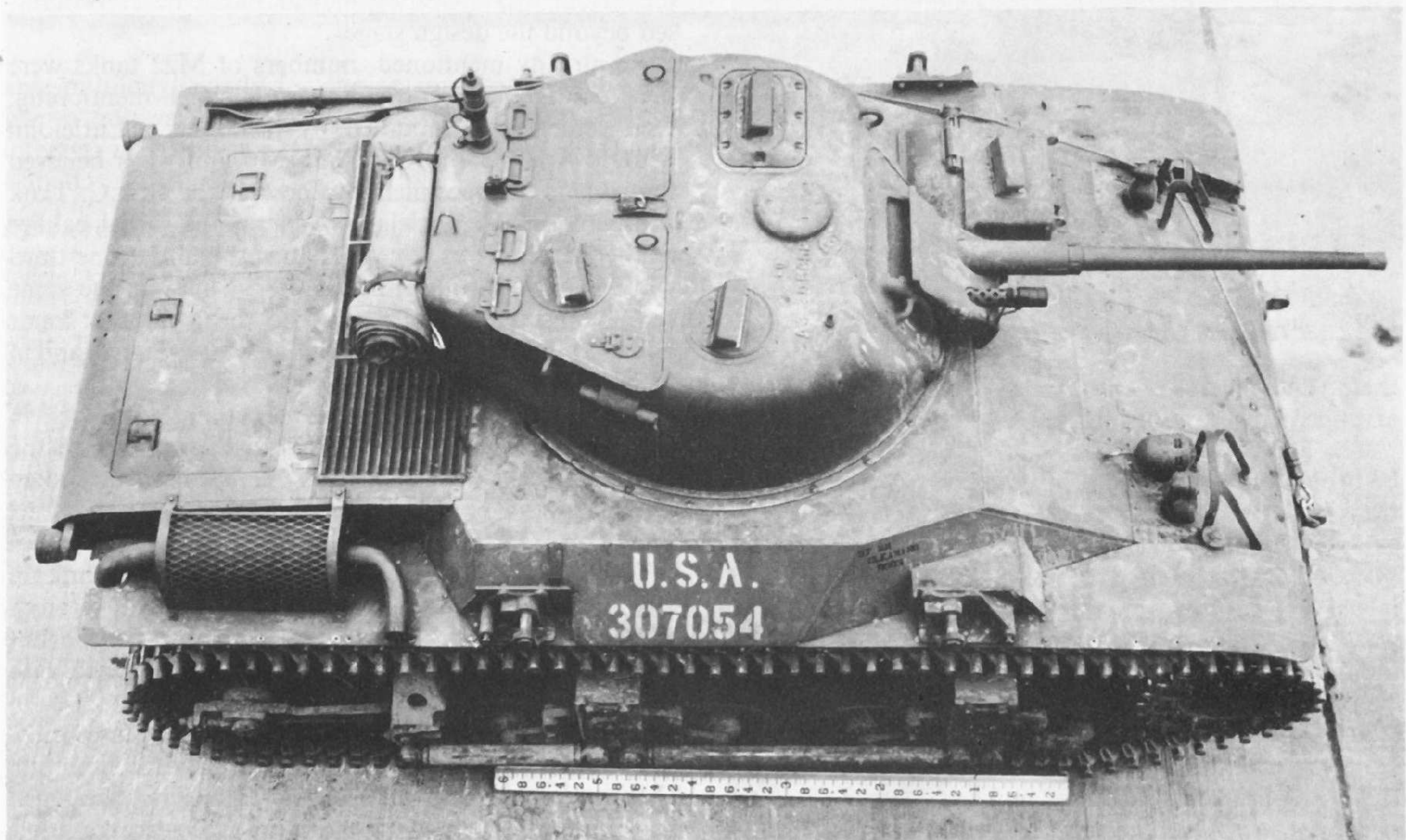
T9E1 Light Tank top showing turret changes and details of hull construction.
