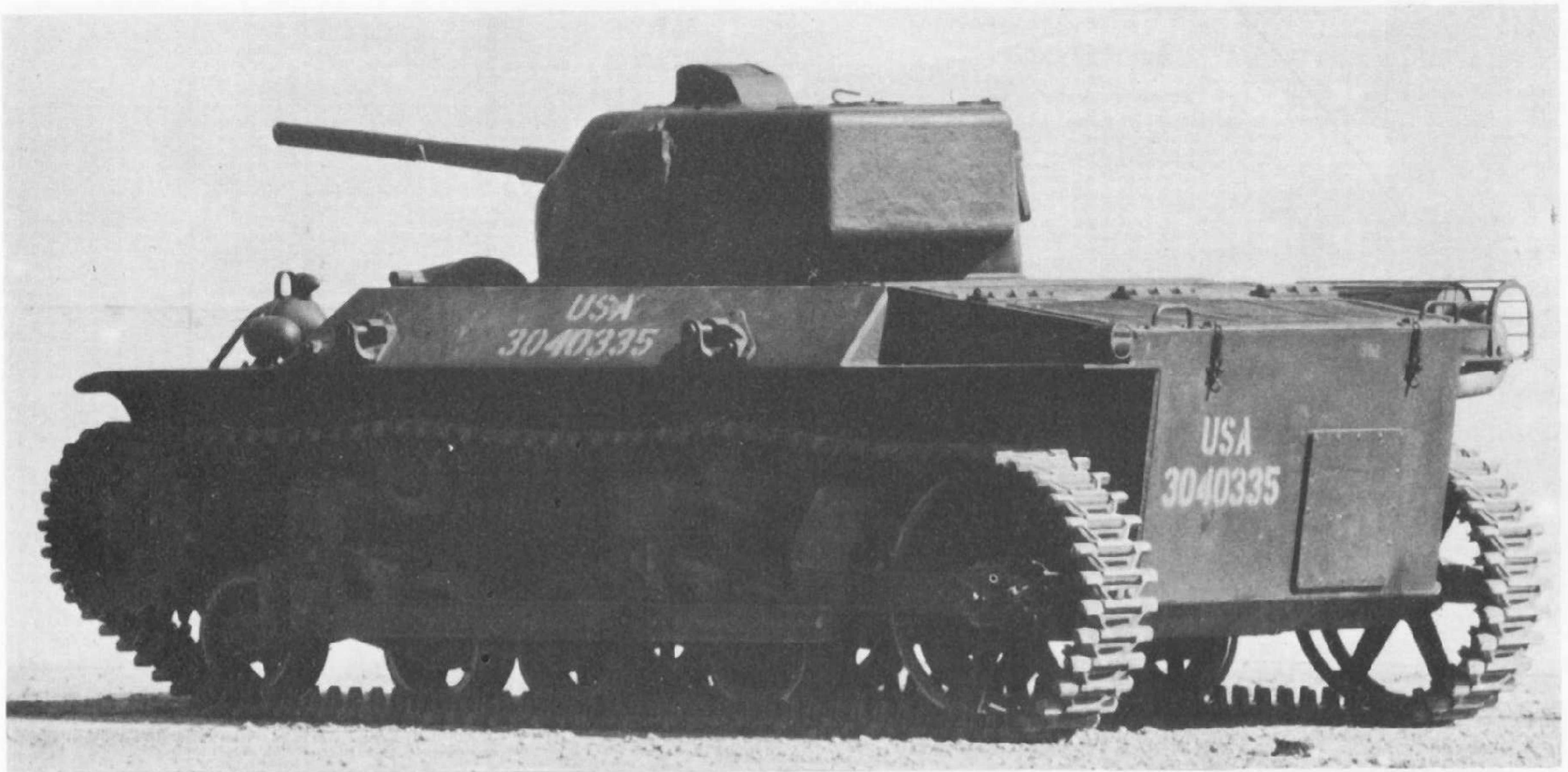
T9 modified to add suspension support beam and showing air carrying brackets.
