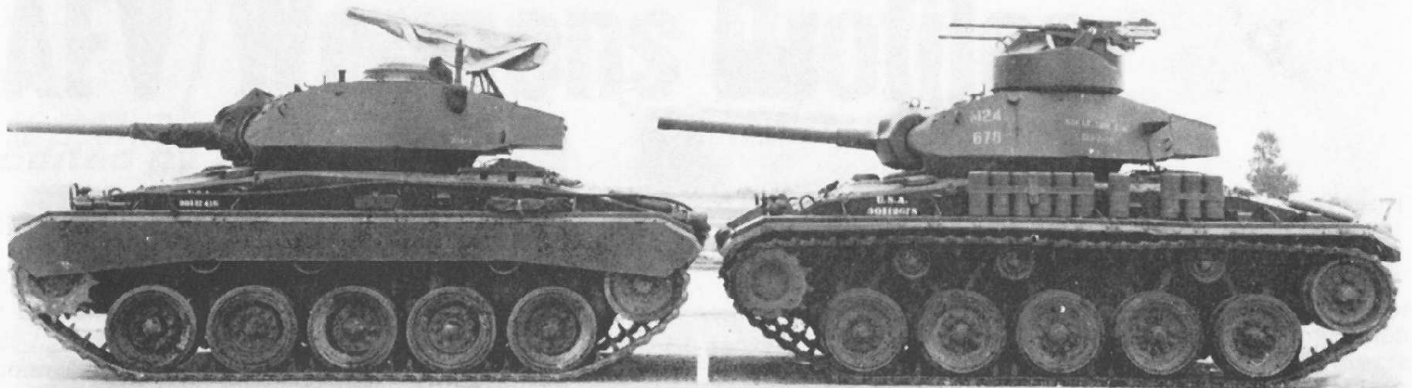
M.24 with T.122 remote control machine gun mount. Weights are placed on the fenders for proving trials.
