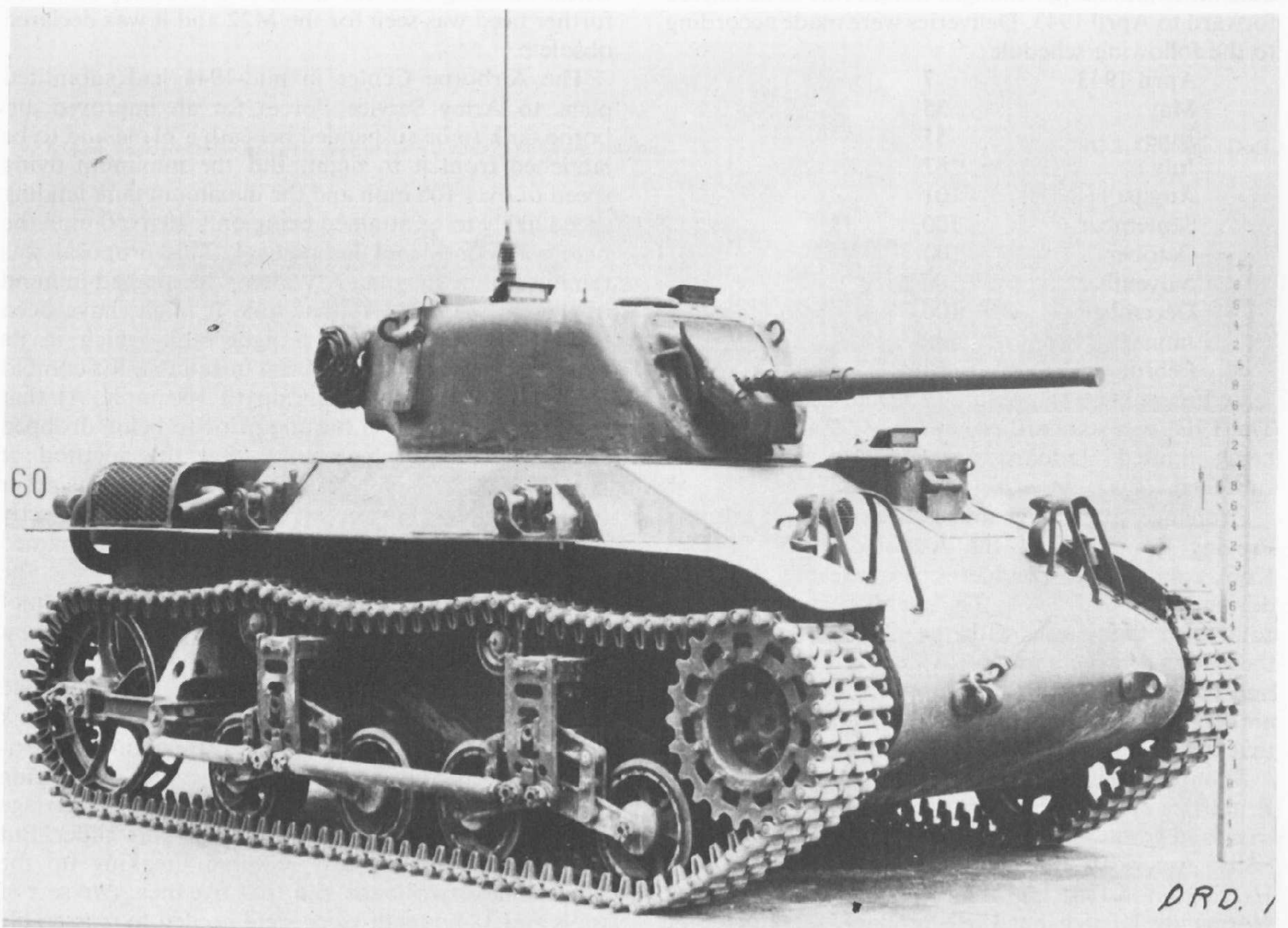
The T9E1 Light Tank with strengthened air carrying brackets, new front end, elimination of bow machine-guns, and lightened suspension units.
