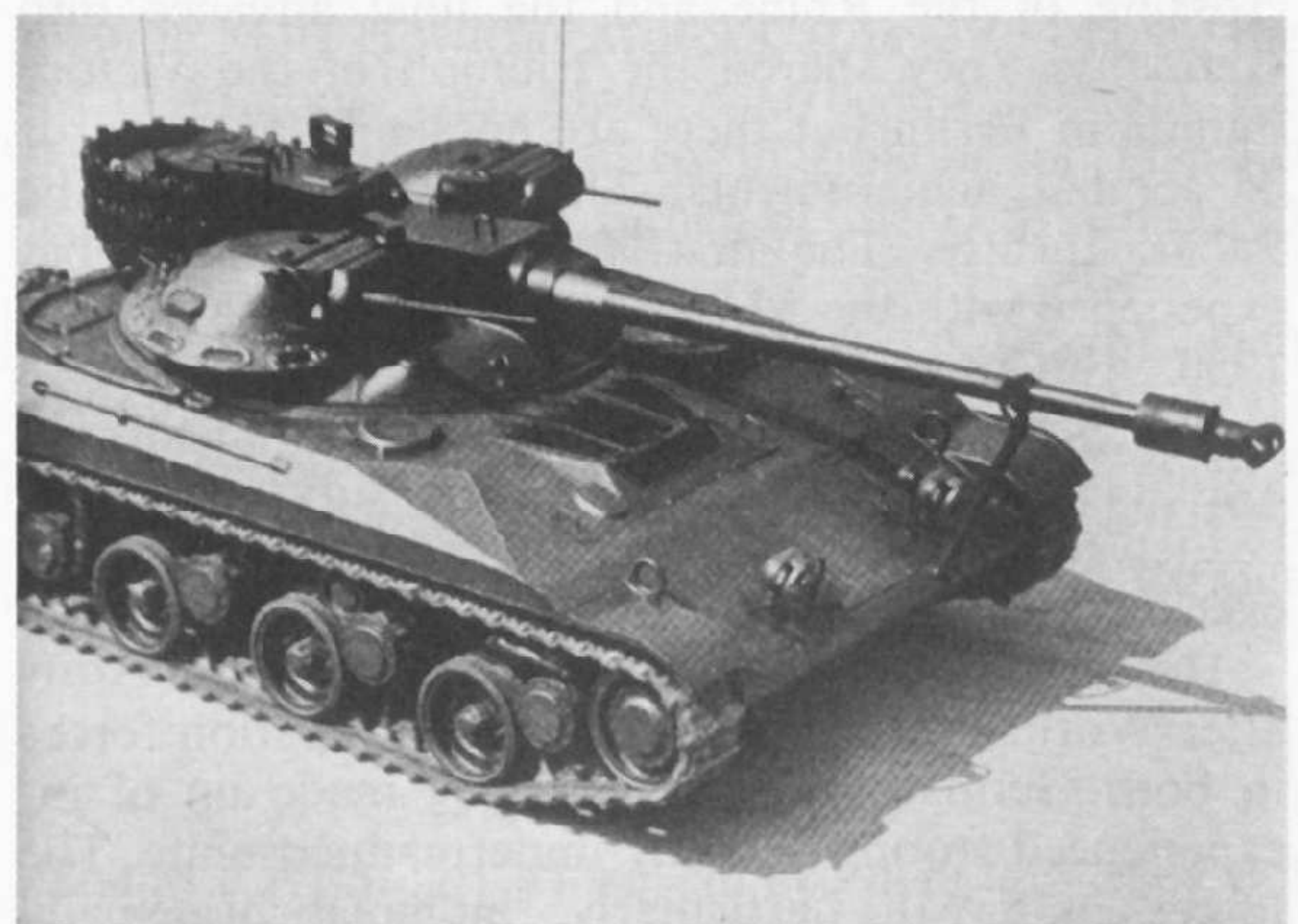
Below: View of the T92 Light Tank showing its cleft turret. As in a conventional turret the gun is elevated on its own, but its depression is achieved by allowing the breech assembly to move up through a large aperture in the roof instead of by having adequate room within the turret. This allows the height of the cleft turret to be considerably lower than that of a conventional turret and thereby reduces its frontal area. But the cleft turret has disadvantages, including the difficulty of sealing it. (Aircraft Armaments Inc.)
