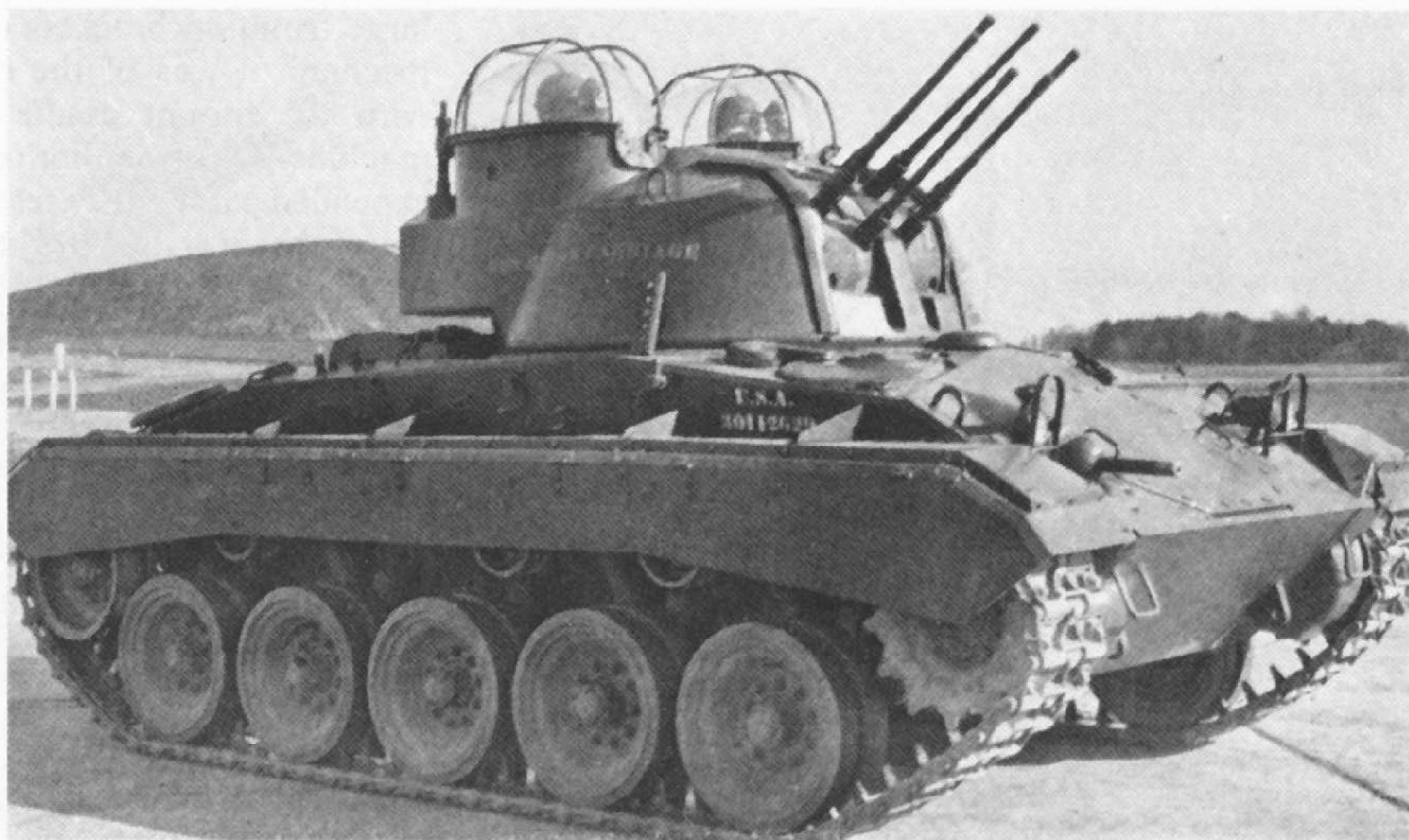
Experimental T.77 E1 Multiple GMC, 1945. (Photo: Icks collection)
