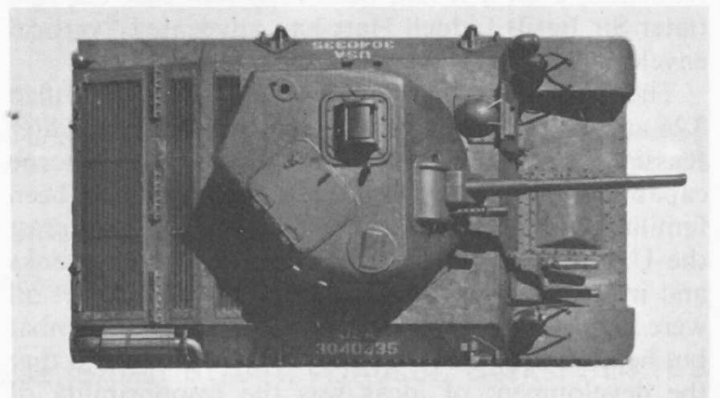
Top view of the T9 after addition of air carrying brackets and showing offset shape of original turret. (General Motors Proving Ground)
