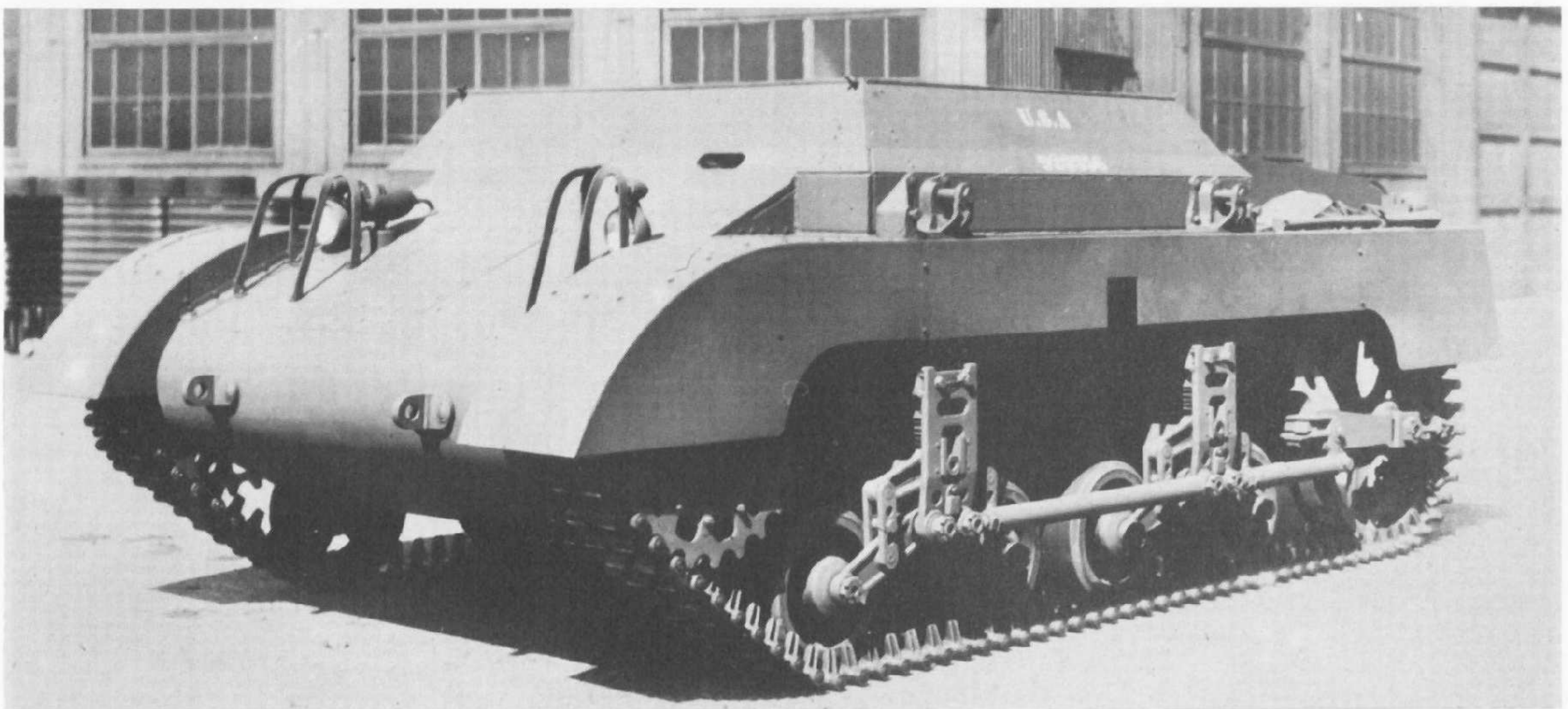
The T18 Cargo Carrier (Airborne) with final M22 suspension and front end but with raised hull.
