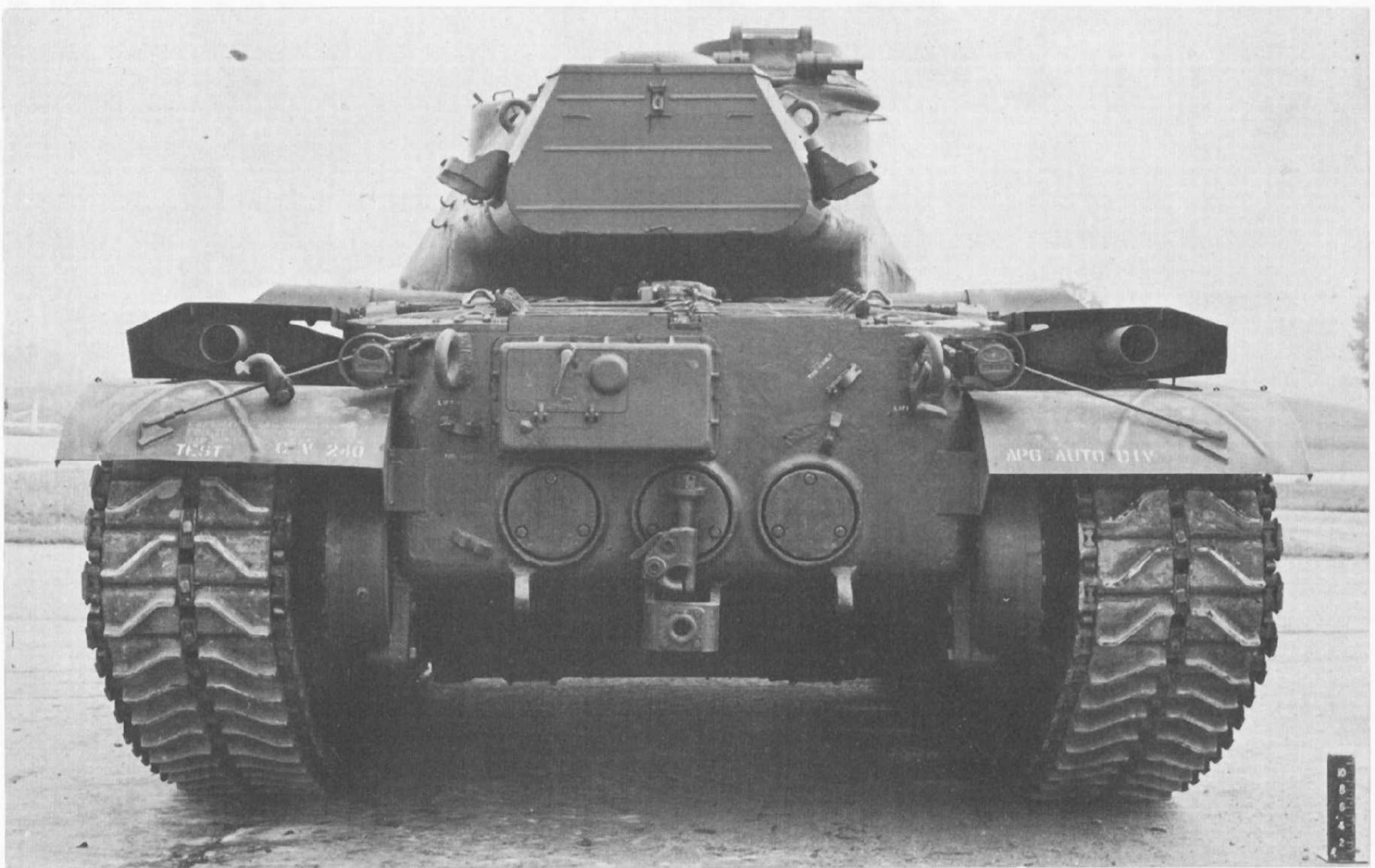
Rear view of early M.47 tank showing location of engine exhaust mufflers, towing pintle, lifting eyes, blackout lights, three round inspection plates, and outside telephone box. (U.S. Ordnance Dept.)
