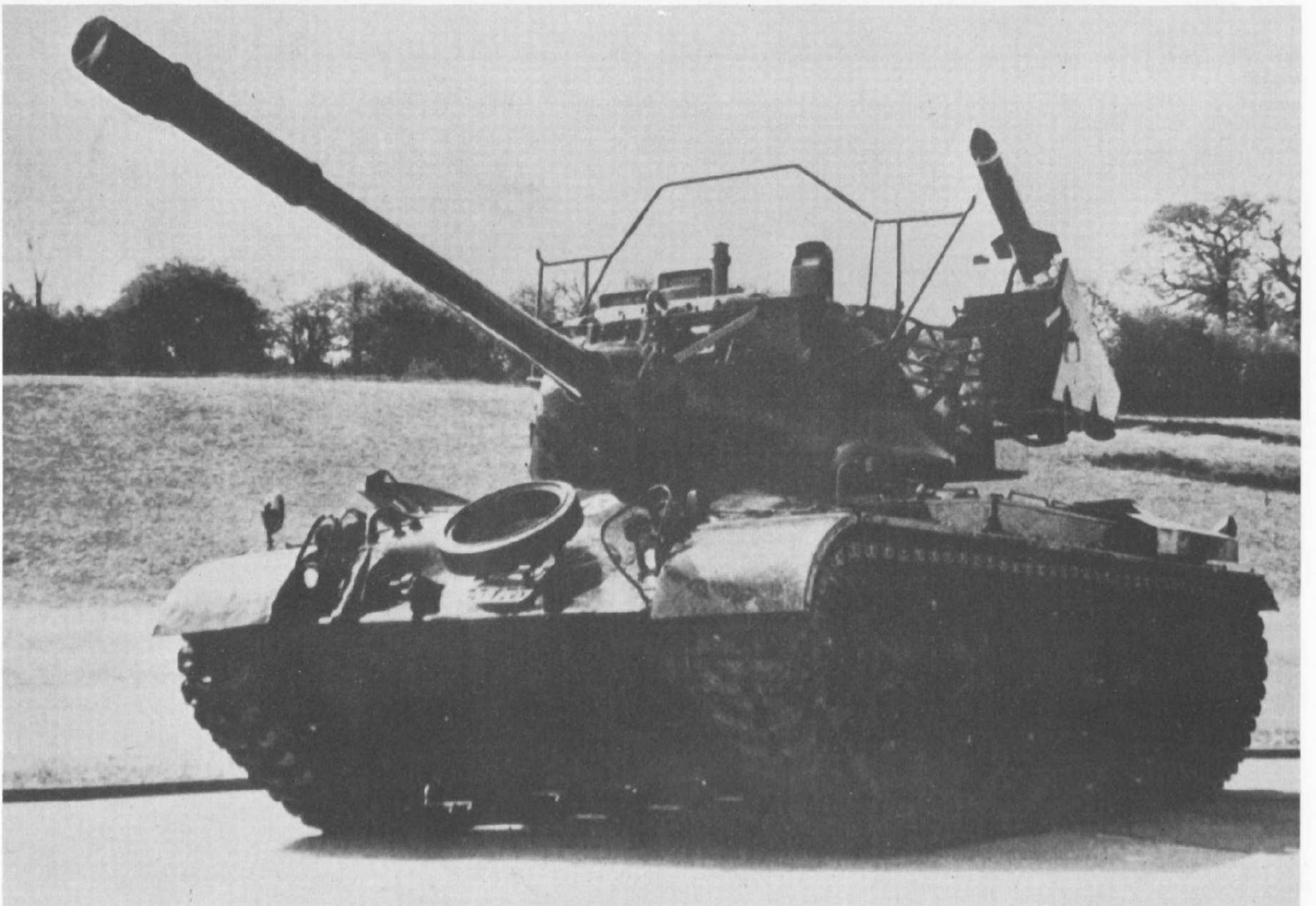
M.47 with mock-ups of BAC Swingfire anti-tank missiles.
