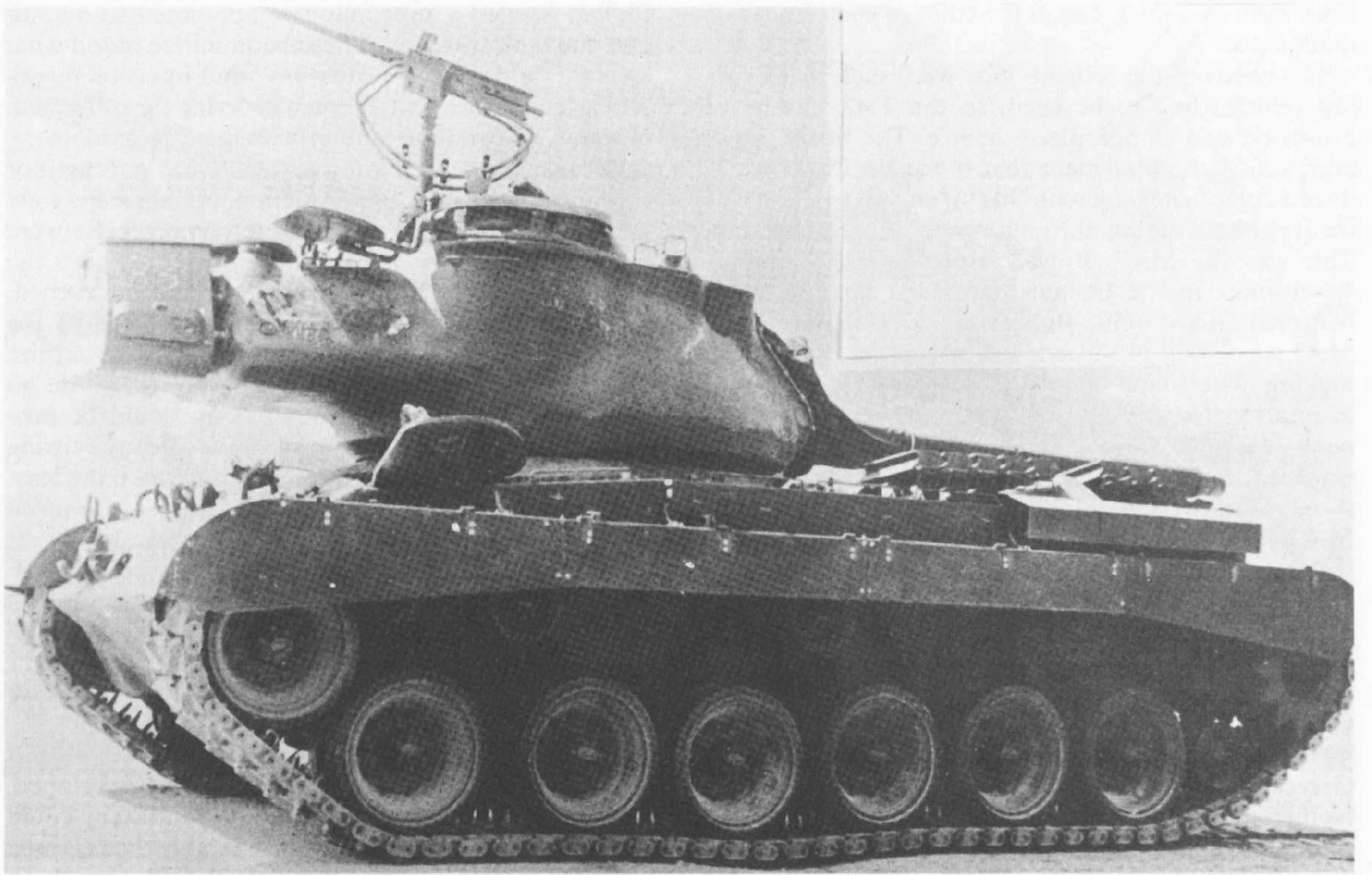
An M.47 tank with turret reversed and fitted with the experimental anti-aircraft cradle mount with handholds for the .50 calibre gun. (Courtesy: S. L. Sola)
