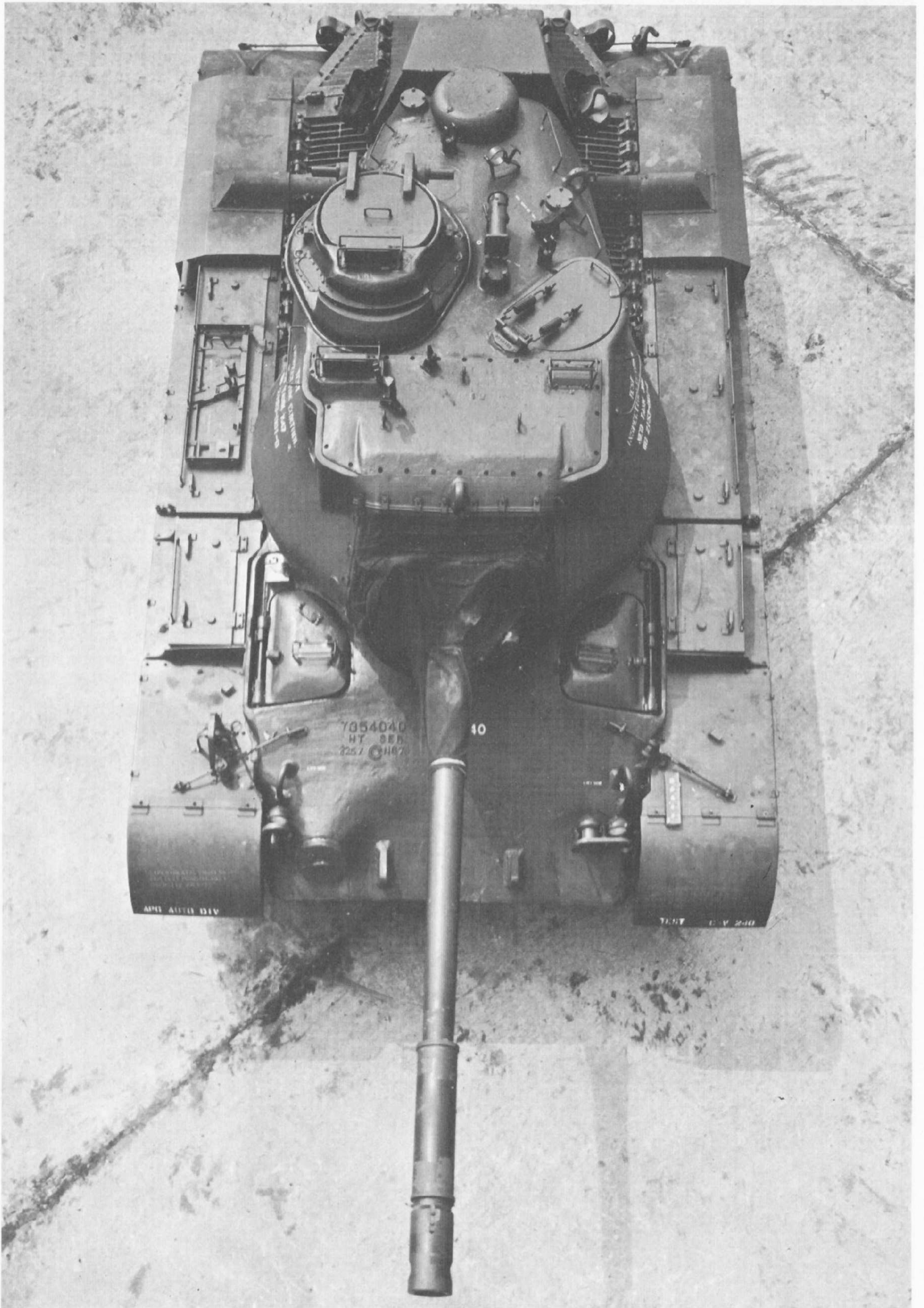
Top view of early M.47 without rangefinder or bow machine-gun.
