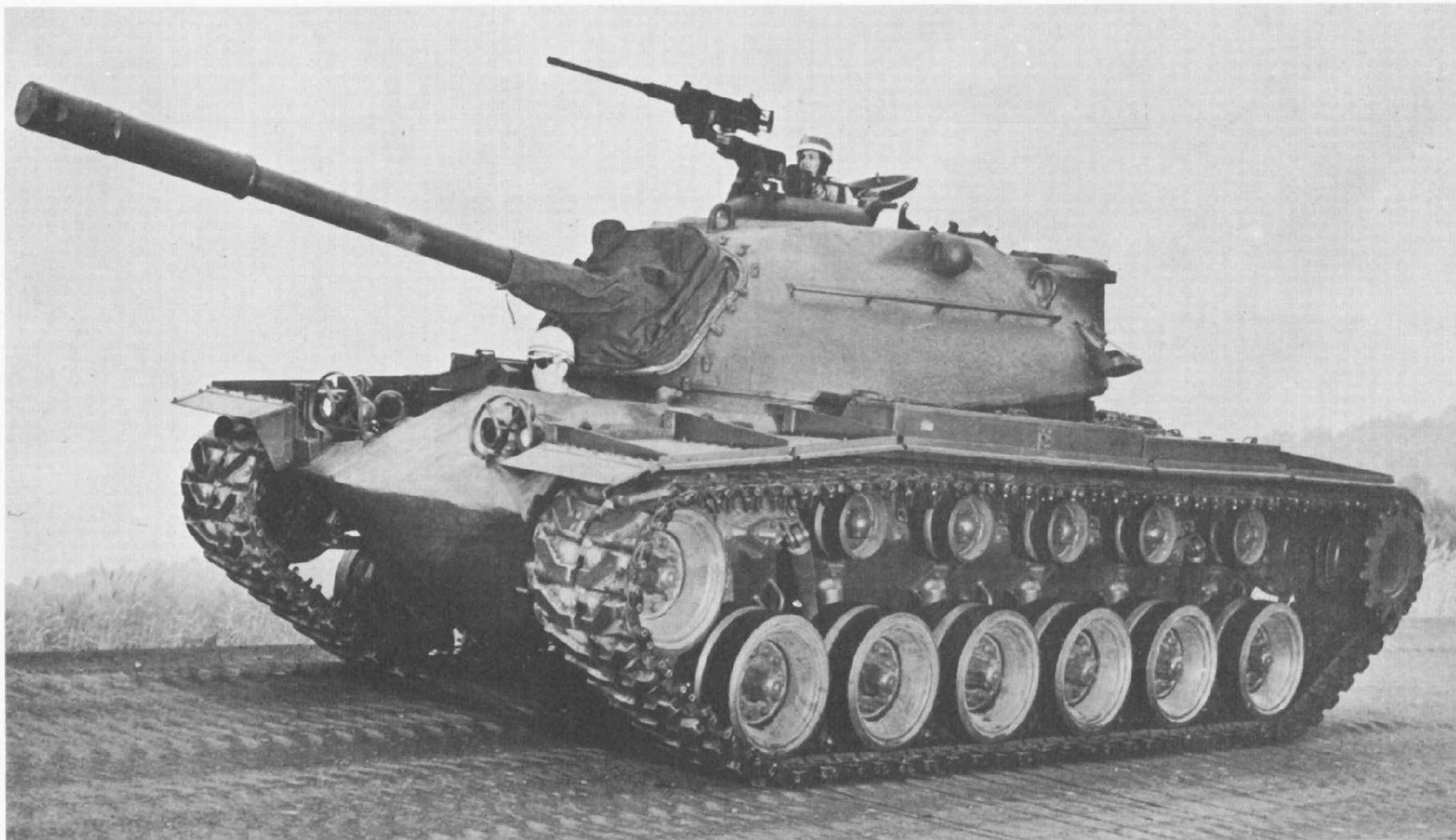
Prototype of the T.48 Medium Tank, showing the ellipsoid turret and hull, which grew out of the M.47 design. (Courtesy Chrysler Corporation)
