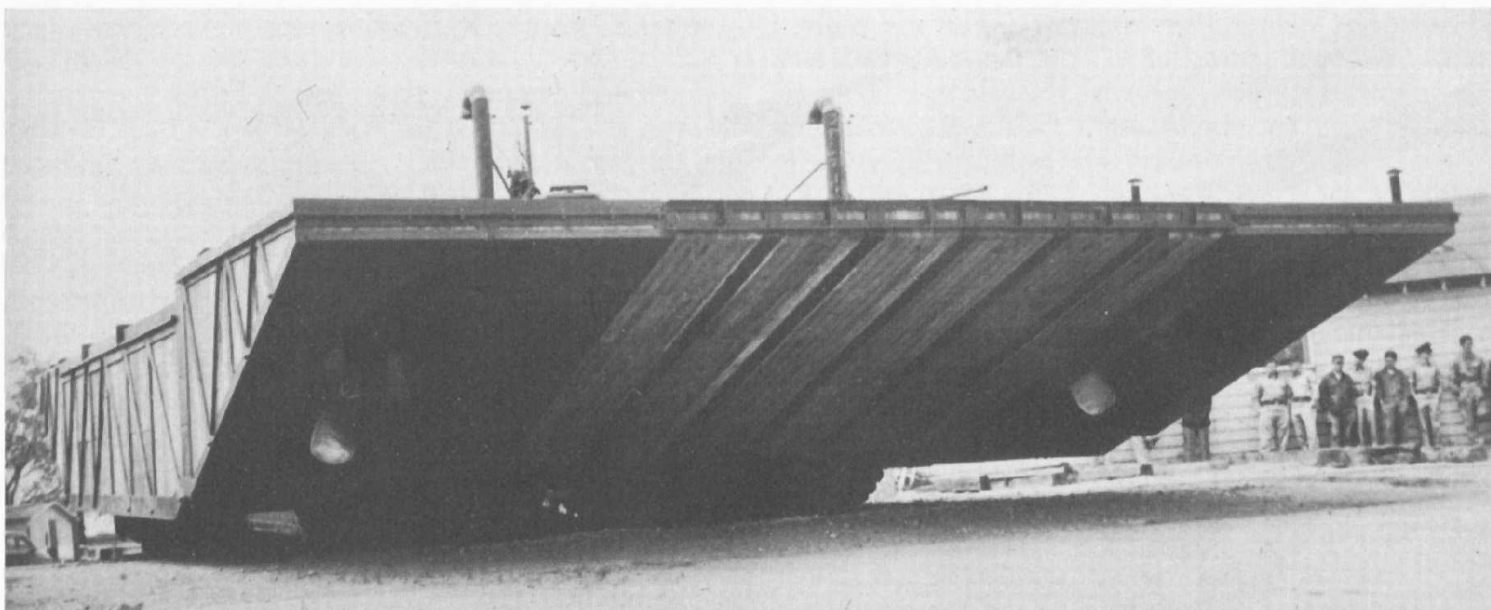
Rear view of T.15 flotation device fitted to an M.47 tank showing the two 36-inch screws and both engine ventilation snorkels. (Courtesy Angersoll Products Div., Borg-Warner Corporation)
