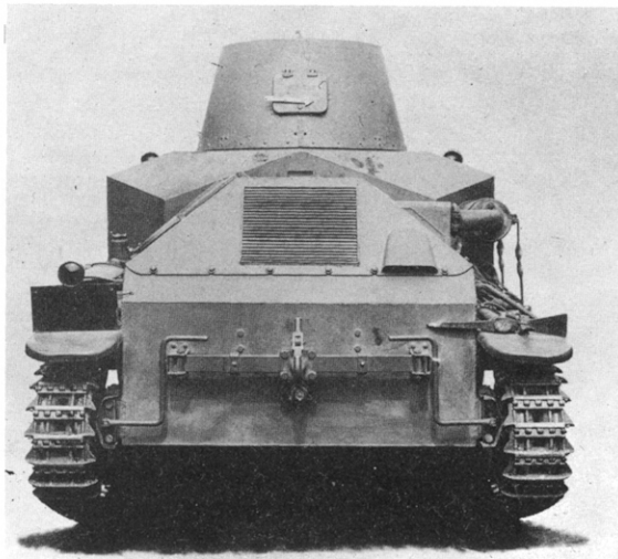
Front and rear views of Type 92 Heavy Combat Car. Although this vehicle was fully tracked and hence was actually a light tank it was called a combat car because of its use by the cavalry.
