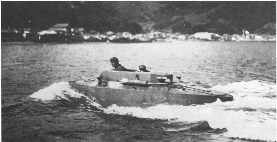
The amphibious half-track afloat.
