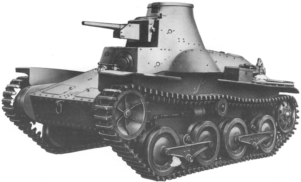
Type 95 Light Tank, Northern Manchuria version, with modified suspension to overcome the severe pitching that resulted when crossing the furrows of kaoliang fields. Note that the bogie arms have been inverted and a small roller has been added to each between the pairs of normal bogie wheels.
