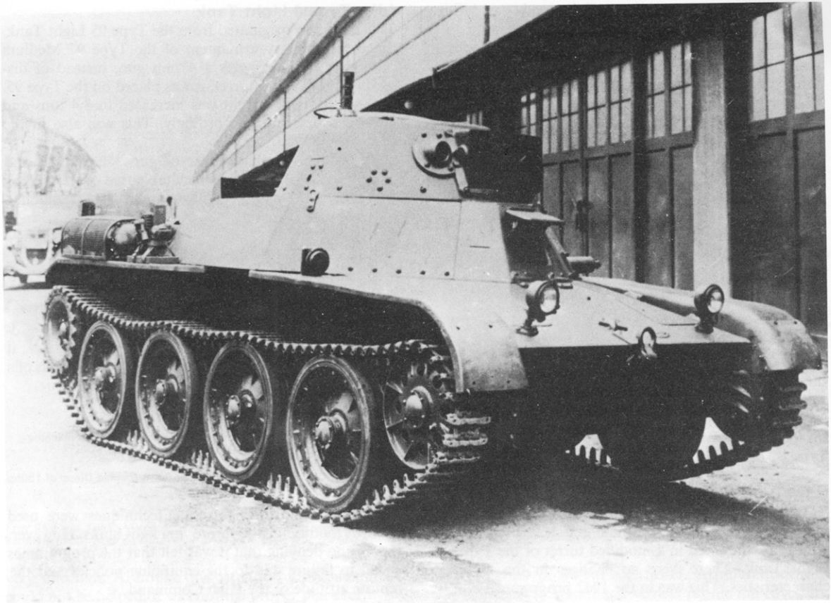
Type 98 Light Tank Model B prototype built by Mitsubishi Heavy Industries in 1938. Note the Christie-type suspension. This tank was rejected in favour of the Hino Model A.
