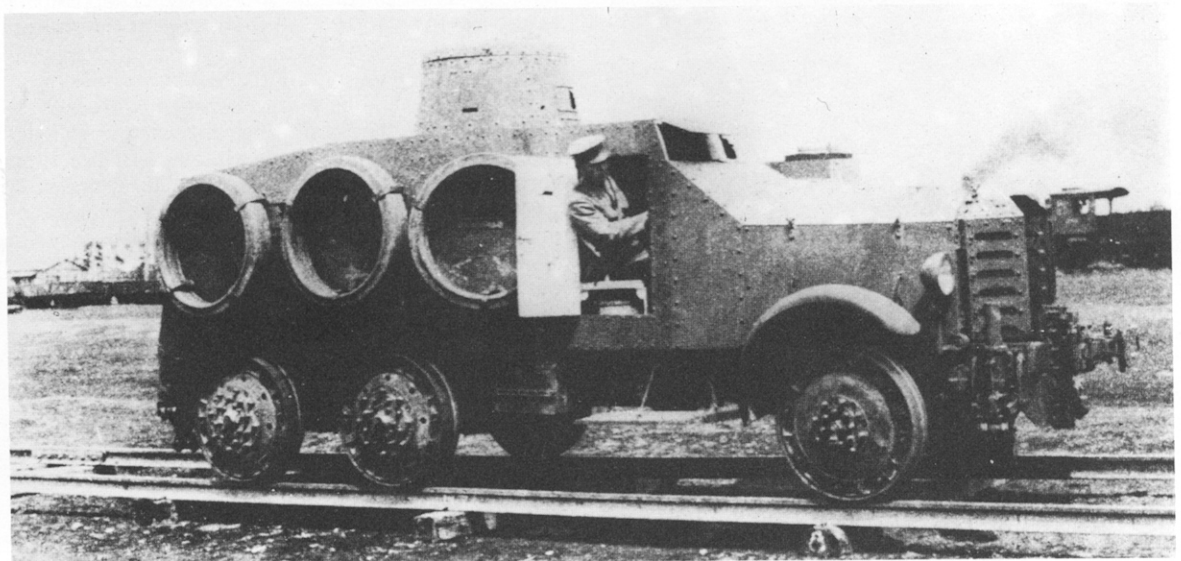
Type 91 Wide-Gauge Tractor. Rubber tyres for road use of vehicle are strapped to the side.
