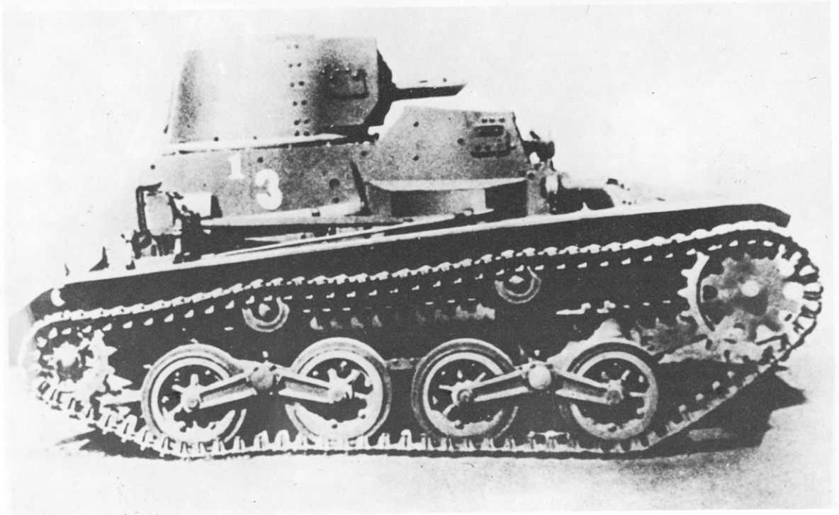
Side view of the prototype Type 94 Tankette built by the Tokyo Gas and Electric Industry (predecessor of Hino Motors) in 1933.
