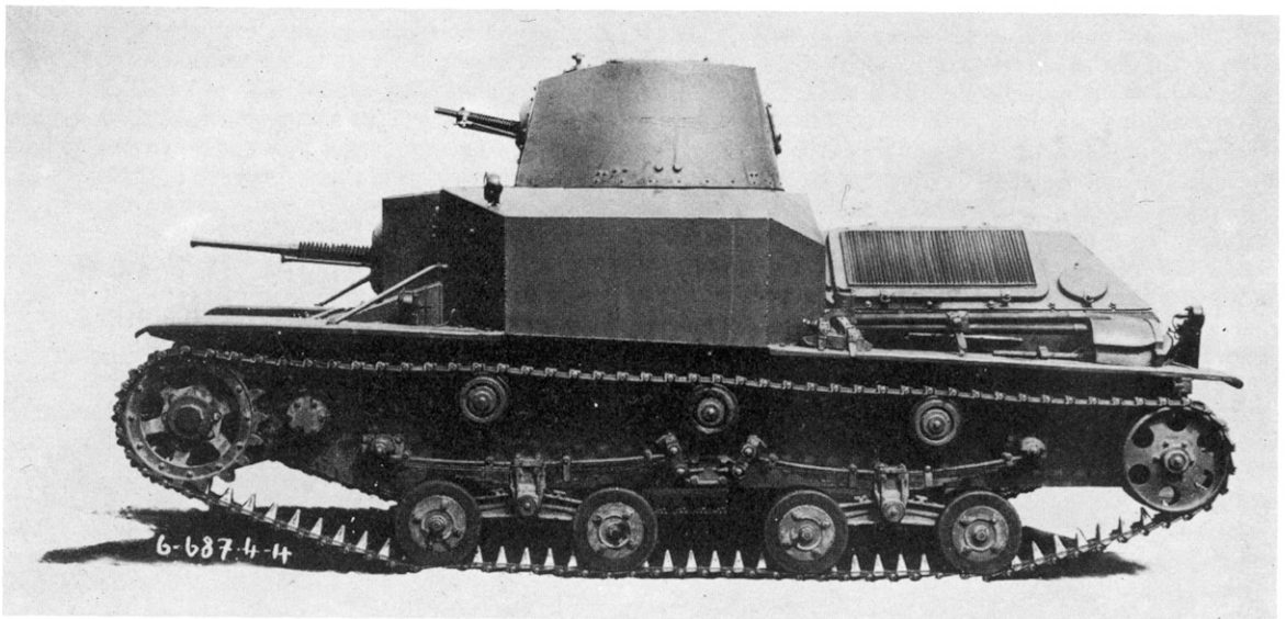
Side view of Type 92 Heavy Combat Car. This is the first version with four bogie wheels each side.
