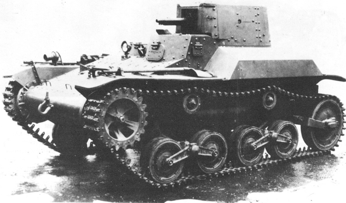
Three-quarter left front view of Type 97 Tankette, first design plan with the driver and the engine side-by-side forward and the turret with its machine-gun located aft. The Tankette was built by Tokyo Motors in 1937; the powerplant was by Ikegai Motors.
