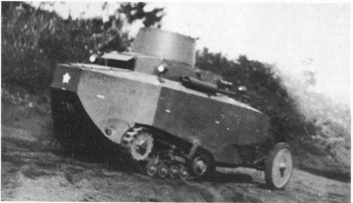
The amphibious half-track had tracks in the front and a pair of wheels aft.
