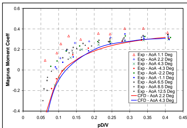
Figure 3. Comparison of computed Magnus moment coefficient versus spin rate with wind tunnel data for boattailed ANSR configuration.
