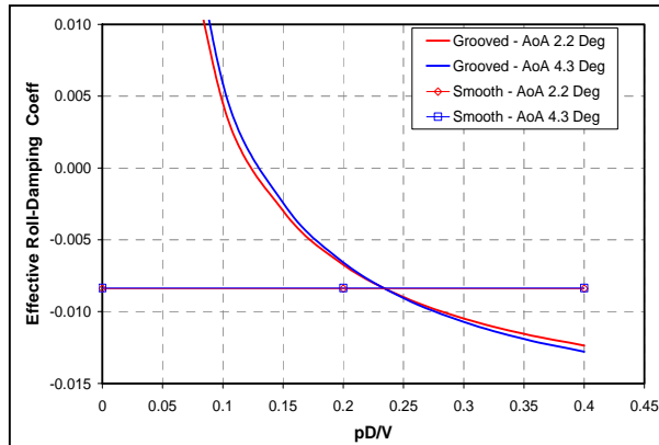
Figure 4. Comparison of the computed effective roll-damping moment coefficient versus spin rate for grooved and smooth boattailed ANSR configuration.
