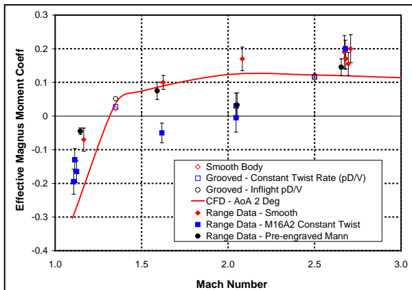
Figure 5. Computed and experimental effective Magnus moment coefficient versus Mach number data for the M193 projectile configurations.
