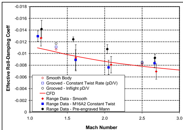
Figure 6. Computed and experimental effective roll-damping coefficient versus Mach number data for the M193 projectile configurations.
