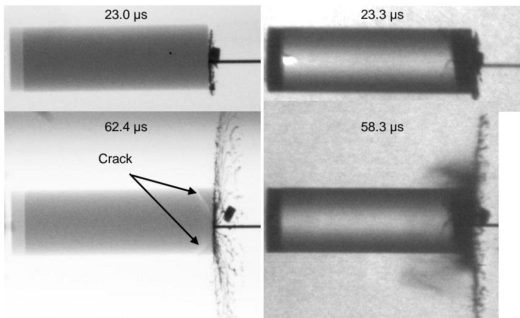
Figure 3. X-ray images (left) and camera pictures (right) for Exp. 10862 ( v_p = 890 m/s); times after impact
