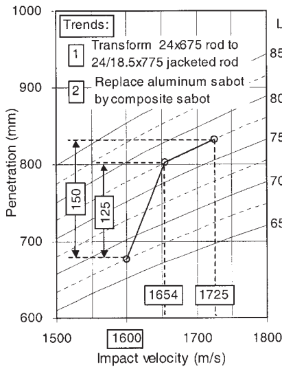
Figure 4. Penetration in RHA (BHN 260/ 60°).
