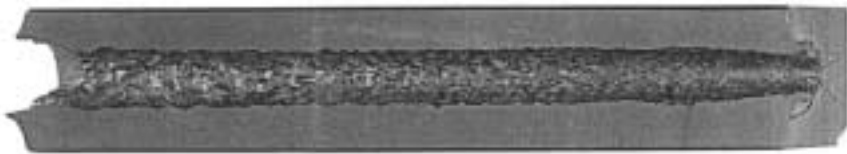
Figure 1. Tungsten rod penetration in a 400 mm thick RHA plate of 260 HB hardness, obliquity 53° NATO (1994 test in Thun).
